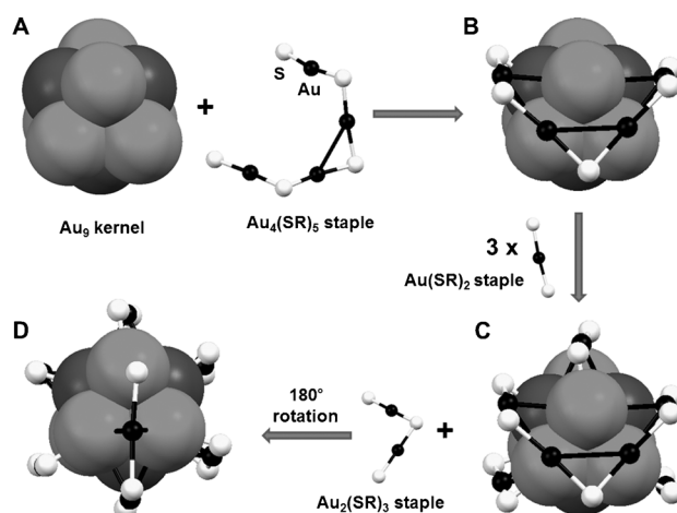
Figure 3. Anatomy of the [\text{Au}_{18}(\text{SC}_6\text{H}_{11})_{14}]^0 nanocluster, starting with the bi-octahedral \text{Au}_9 kernel (A), to which one tetrameric staple motif is added giving (B), followed by addition of three monomeric staples to give (C), and finally addition of a dimeric staple motif yields the complete structure [\text{Au}_{18}(\text{SC}_6\text{H}_{11})_{14}] (D). (large spheres = Au in the kernel; dark small spheres = Au in the staples; light gray spheres = S; carbon tails of thiolates are omitted for clarity).
